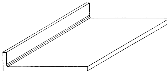
KCT-2 1 1/4" Thick coved plastic laminate counter top with 3/4" backsplash 4" high, 24" deep
