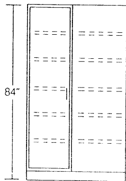
KTBR-4884 Fixed right panel
