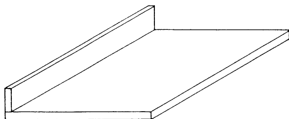
KCT-1 1 1/4" Thick plastic laminate counter top with 3/4" backsplash 4" high, 24" deep
