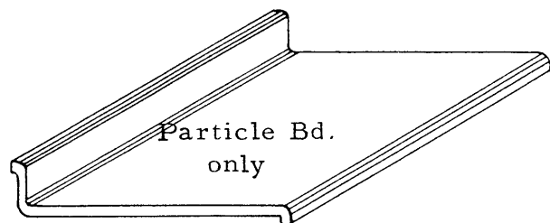
KCT-3 3/4" Thick coved plastic laminate counter top with bullnose edge and 4" splash 25 1/4" deep
