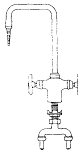
93310 Hot and Cold Water Gooseneck with Aerator Requires 1 hole punch sink
